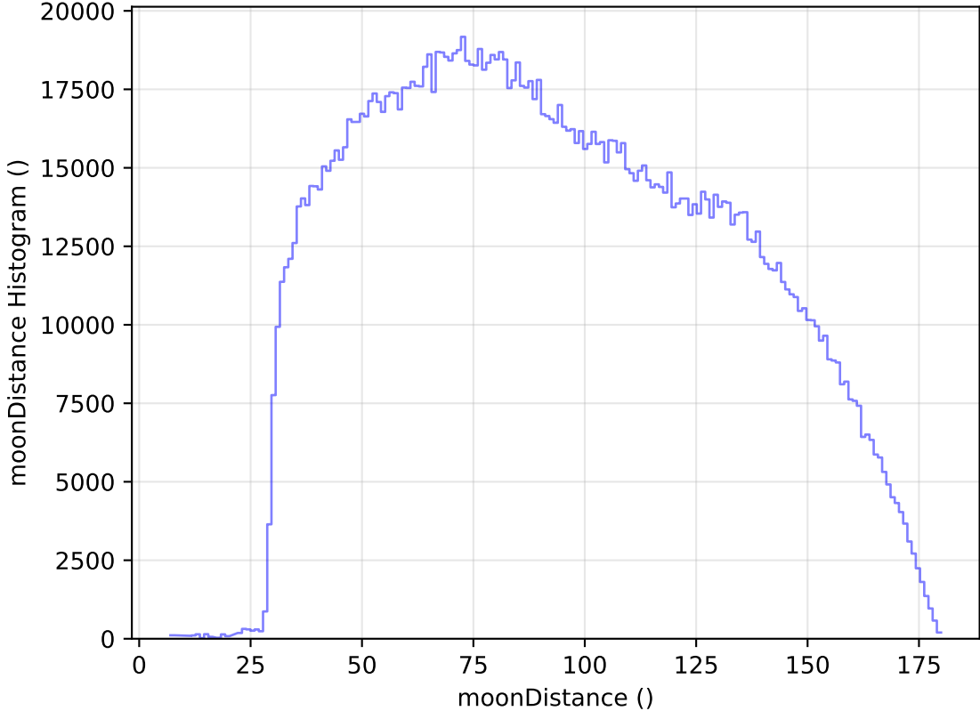
noroll_mjdp365_v3.4_10yrs All sky all bands: moonDistance Histogram
