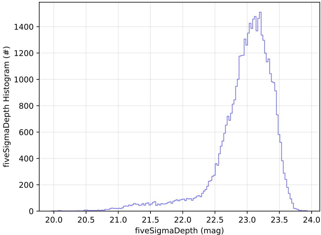
noroll_mjdp365_v3.4_10yrs Yr 1 z band: fiveSigmaDepth Histogram
