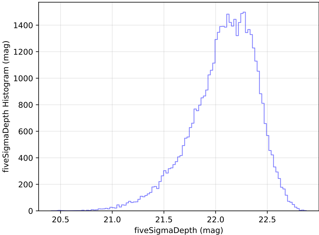
noroll_mjdp365_v3.4_10yrs Yr 1 y band: fiveSigmaDepth Histogram
