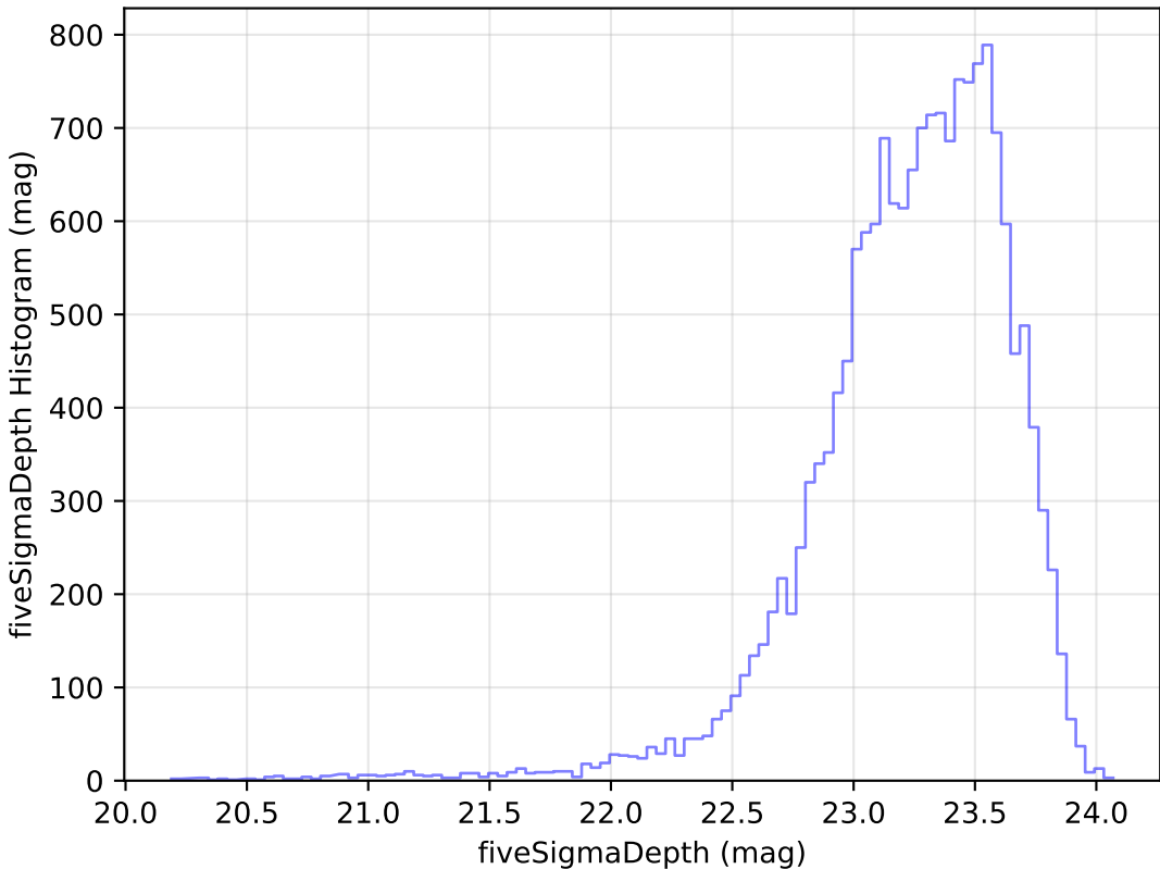
noroll_mjdp365_v3.4_10yrs Yr 1 u band: fiveSigmaDepth Histogram
