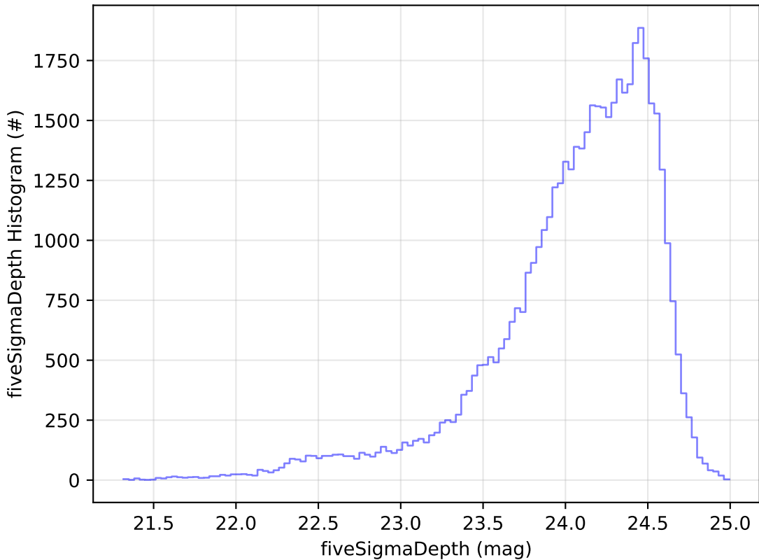
noroll_mjdp365_v3.4_10yrs Yr 1 r band: fiveSigmaDepth Histogram
