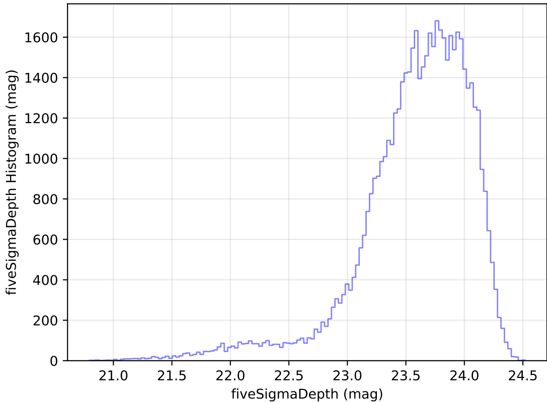
noroll_mjdp365_v3.4_10yrs Yr 1 i band: fiveSigmaDepth Histogram
