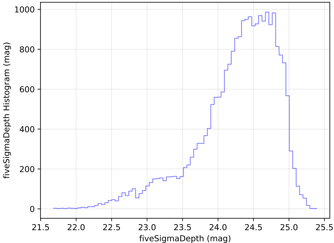
noroll_mjdp365_v3.4_10yrs Yr 1 g band: fiveSigmaDepth Histogram
