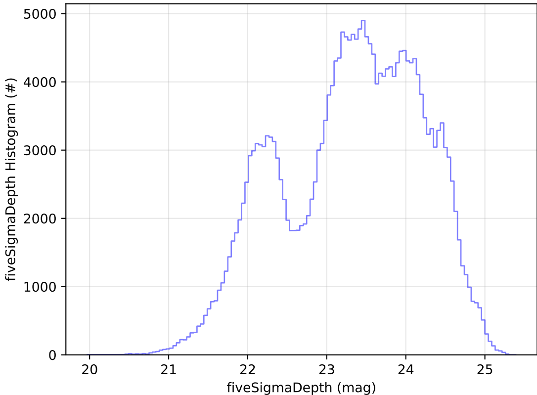
noroll_mjdp365_v3.4_10yrs Yr 1 all bands: fiveSigmaDepth Histogram
