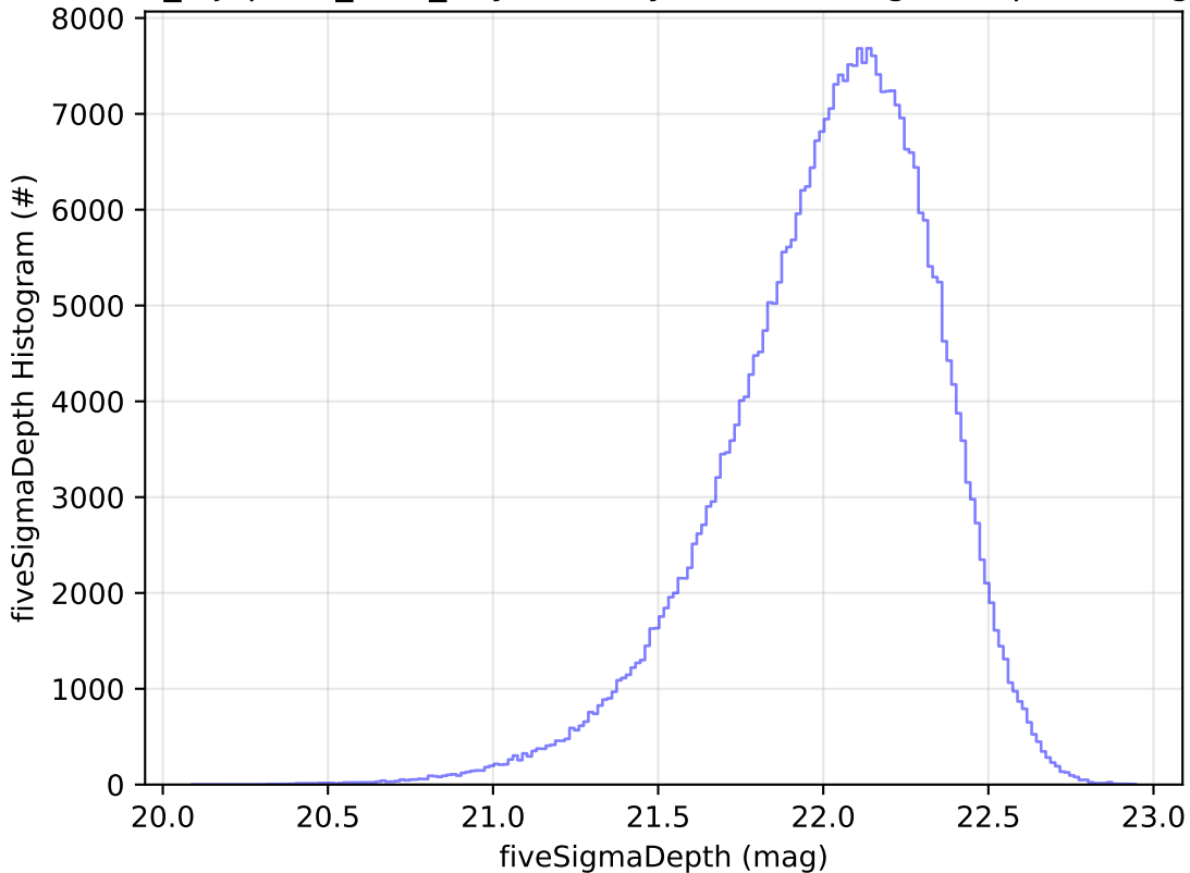
noroll_mjdp365_v3.4_10yrs WFD y band: fiveSigmaDepth Histogram
