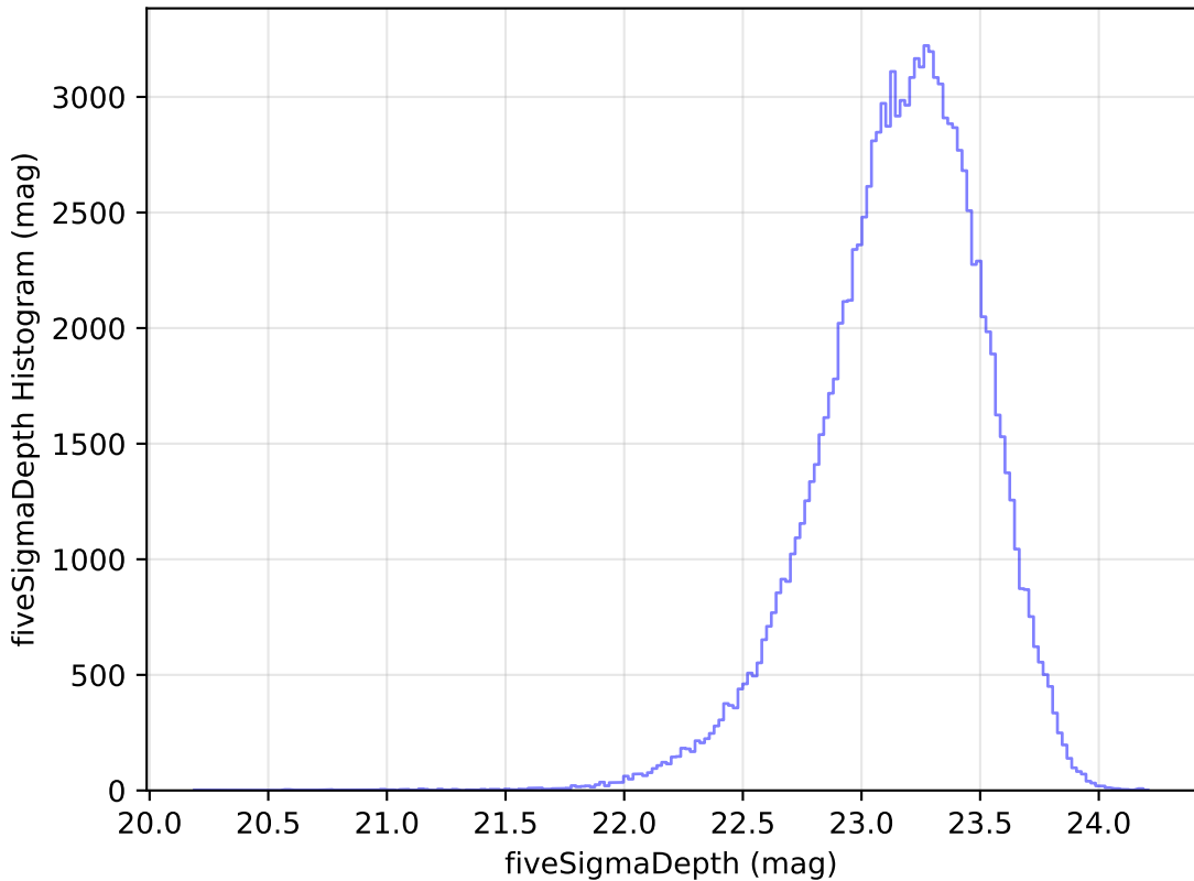
noroll_mjdp365_v3.4_10yrs WFD u band: fiveSigmaDepth Histogram
