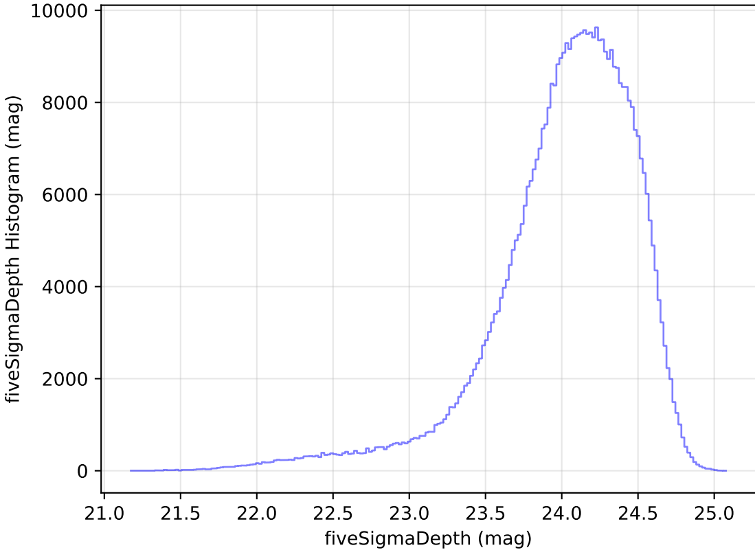
noroll_mjdp365_v3.4_10yrs WFD r band: fiveSigmaDepth Histogram
