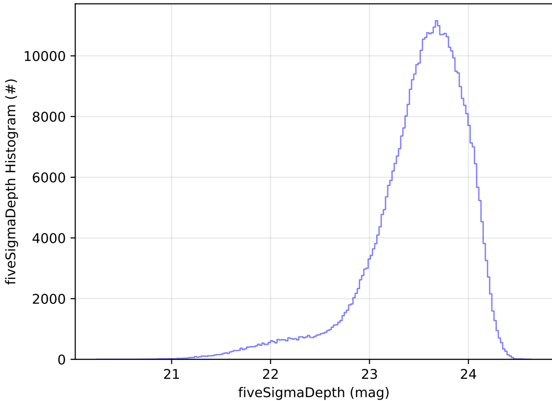
noroll_mjdp365_v3.4_10yrs WFD i band: fiveSigmaDepth Histogram
