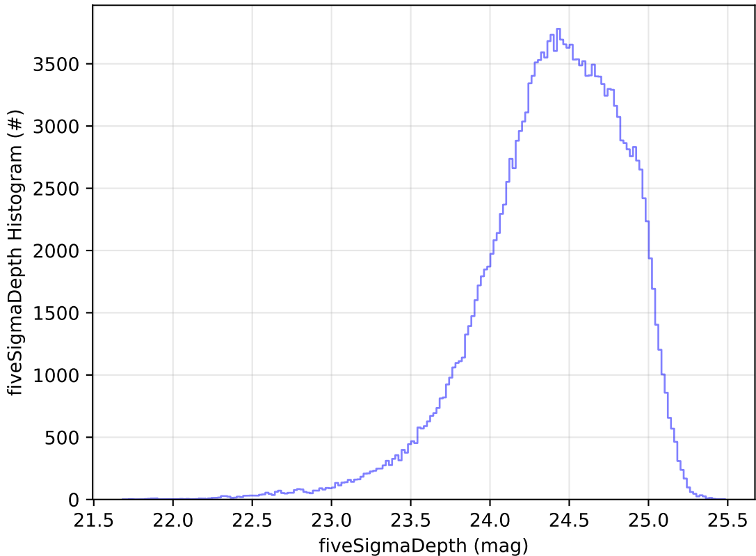
noroll_mjdp365_v3.4_10yrs WFD g band: fiveSigmaDepth Histogram
