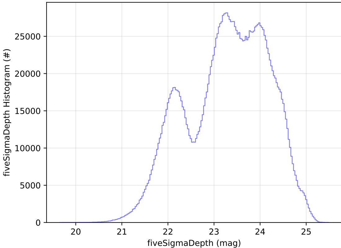
noroll_mjdp365_v3.4_10yrs WFD all bands: fiveSigmaDepth Histogram
