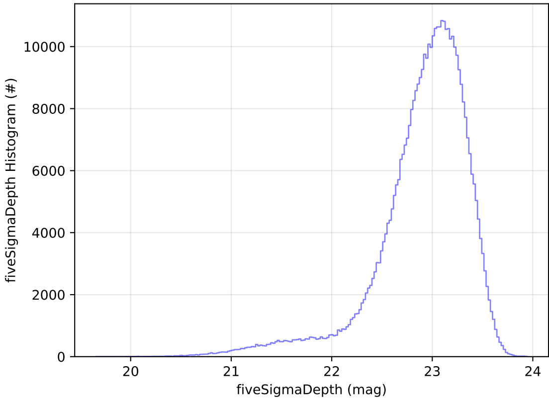
noroll_mjdp365_v3.4_10yrs All sky z band: fiveSigmaDepth Histogram
