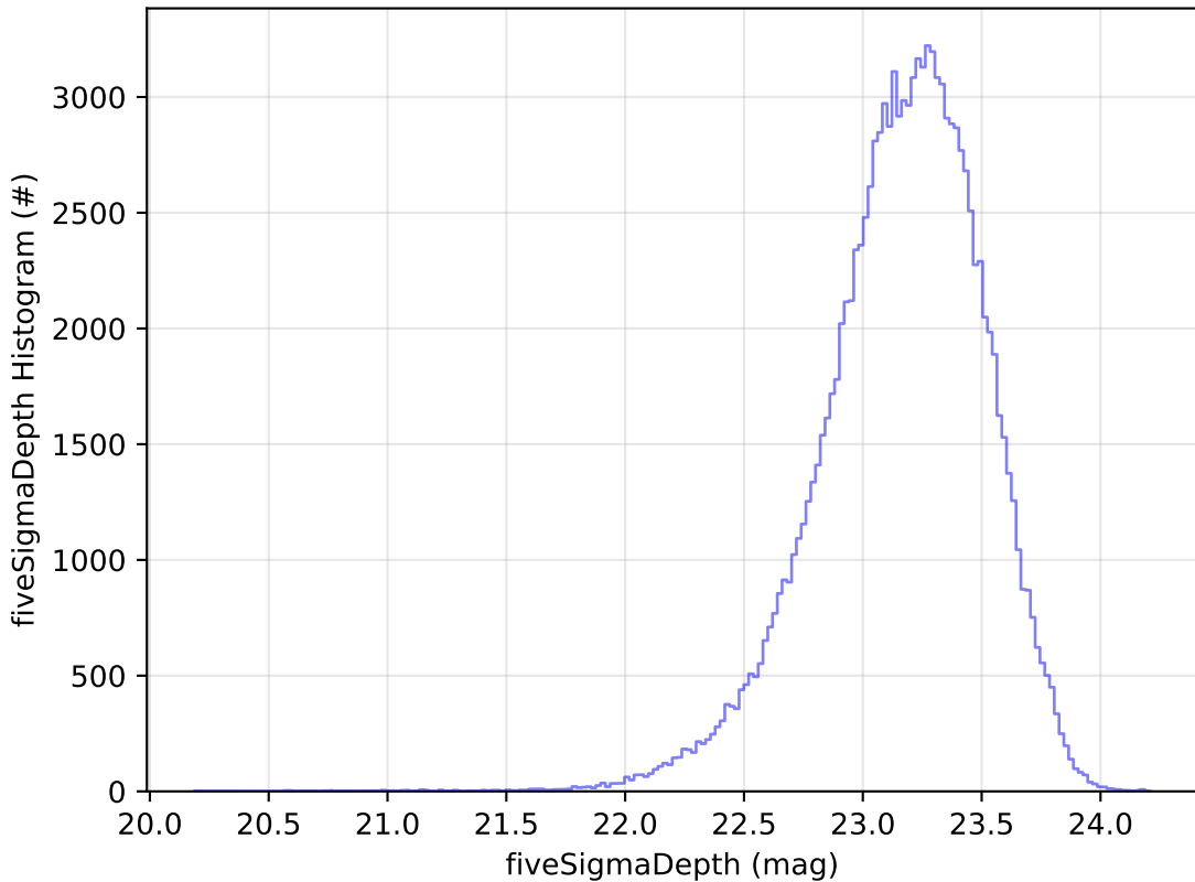
noroll_mjdp365_v3.4_10yrs All sky u band: fiveSigmaDepth Histogram
