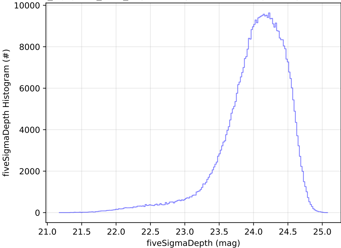
noroll_mjdp365_v3.4_10yrs All sky r band: fiveSigmaDepth Histogram
