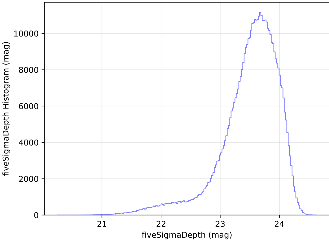
noroll_mjdp365_v3.4_10yrs All sky i band: fiveSigmaDepth Histogram
