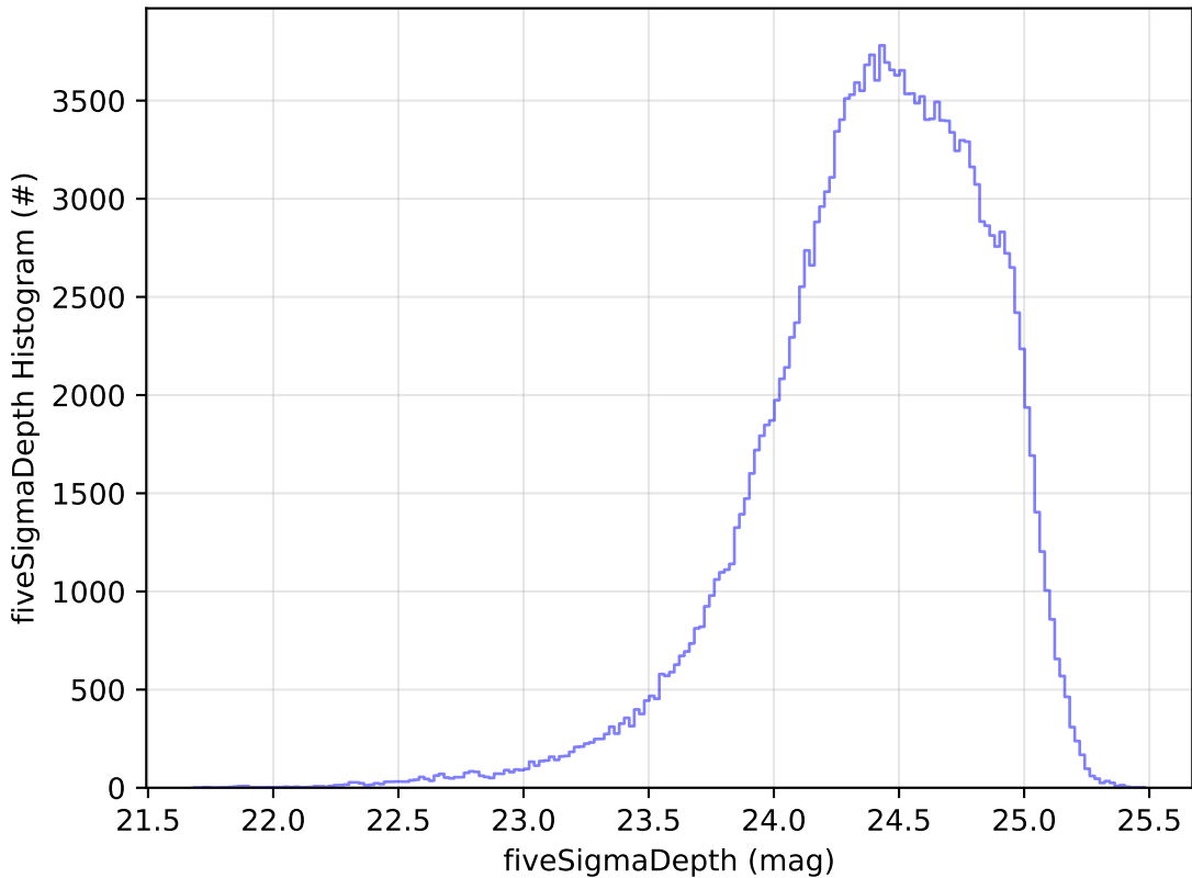
noroll_mjdp365_v3.4_10yrs All sky g band: fiveSigmaDepth Histogram
