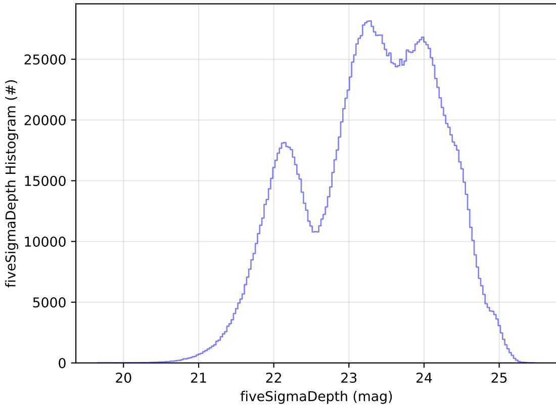
noroll_mjdp365_v3.4_10yrs All sky all bands: fiveSigmaDepth Histogram
