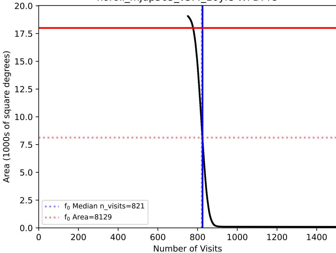
noroll_mjdp365_v3.4_10yrs WFD: f0
