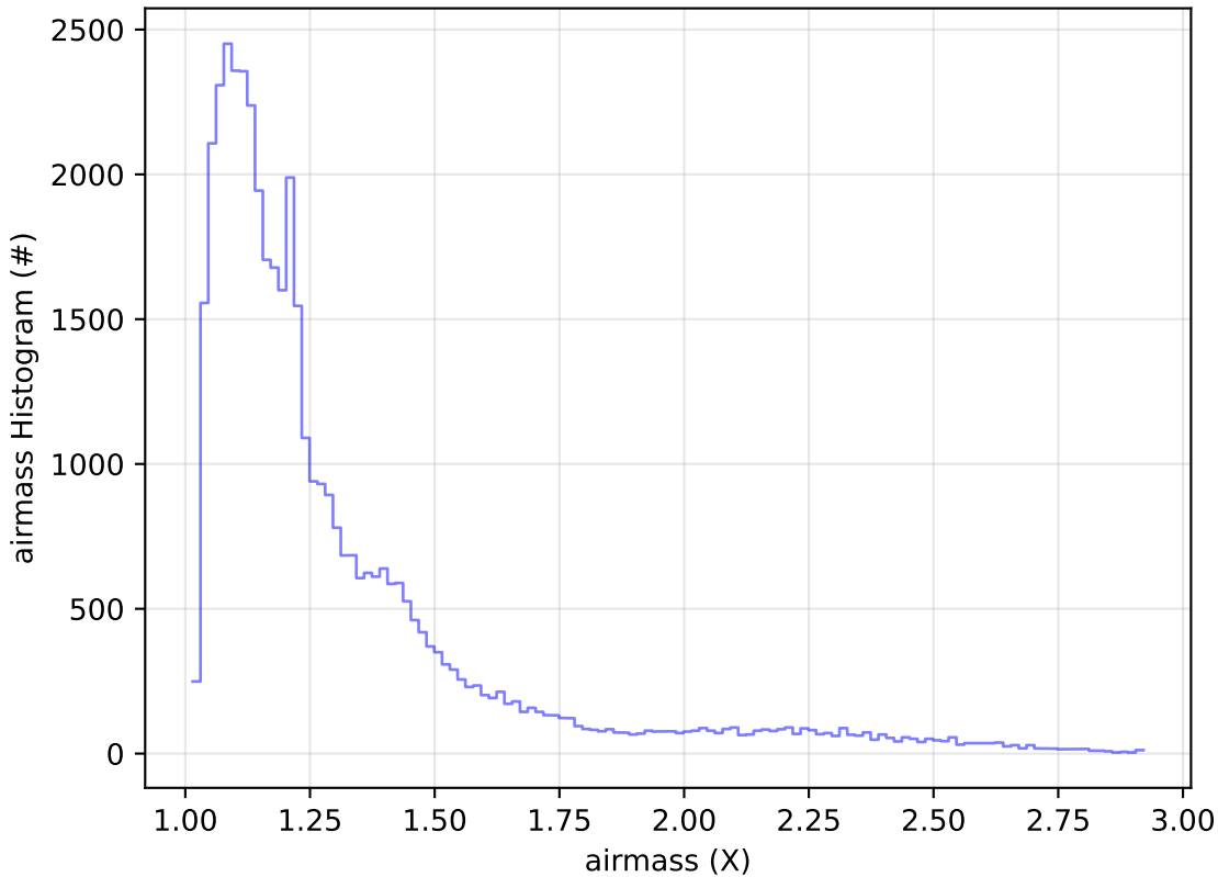
noroll_mjdp365_v3.4_10yrs Yr 1 z band: airmass Histogram
