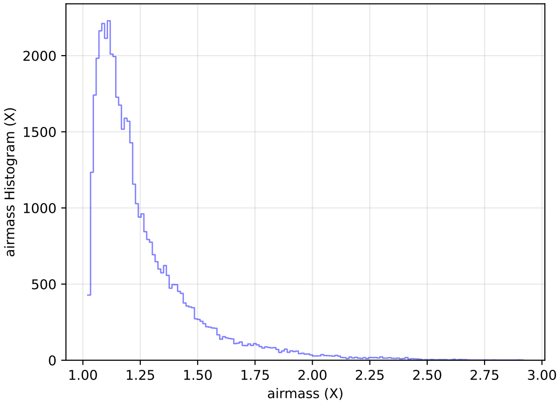
noroll_mjdp365_v3.4_10yrs Yr 1 y band: airmass Histogram
