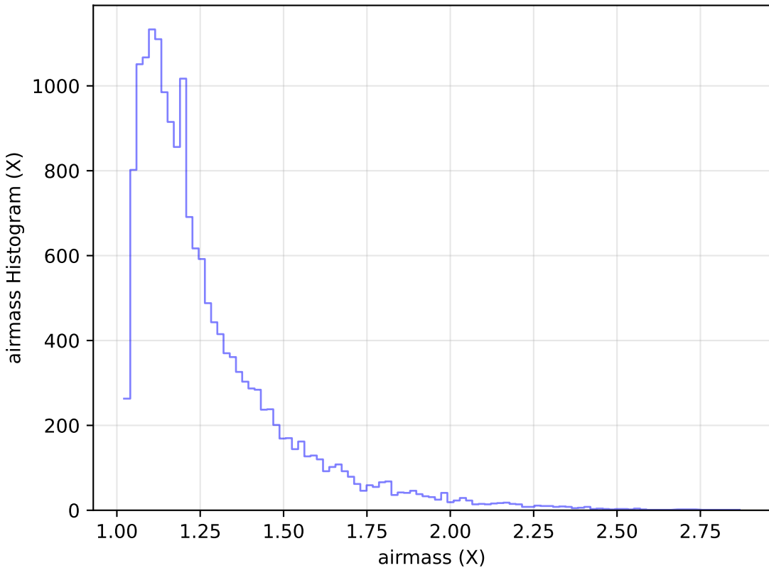
noroll_mjdp365_v3.4_10yrs Yr 1 u band: airmass Histogram
