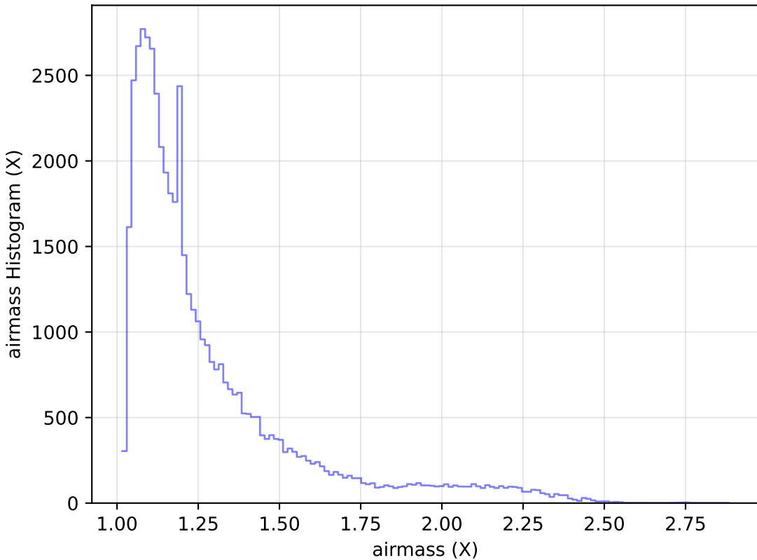
noroll_mjdp365_v3.4_10yrs Yr 1 r band: airmass Histogram
