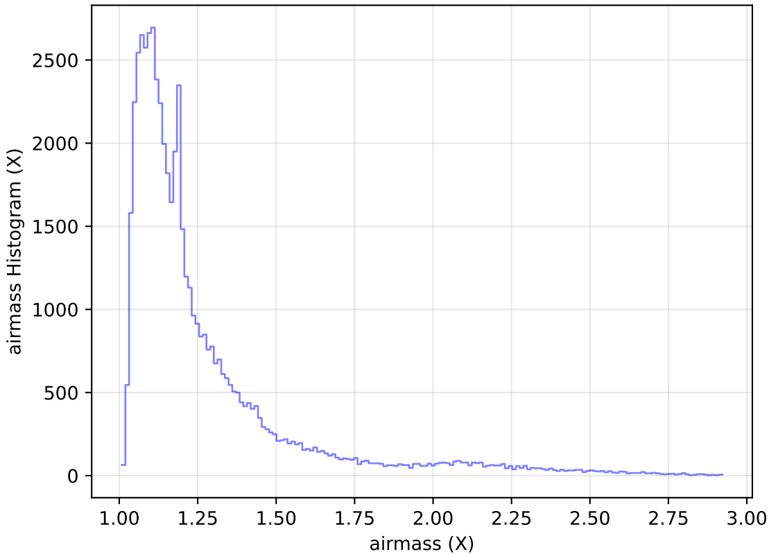
noroll_mjdp365_v3.4_10yrs Yr 1 i band: airmass Histogram
