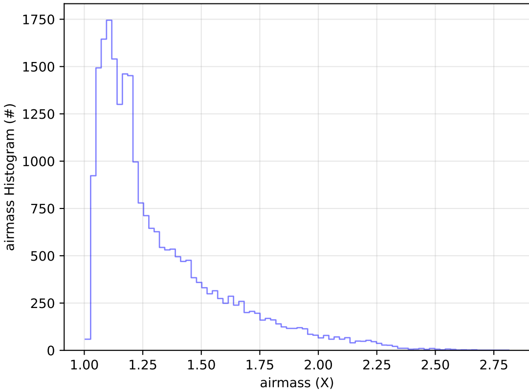
noroll_mjdp365_v3.4_10yrs Yr 1 g band: airmass Histogram
