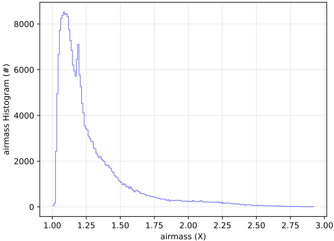
noroll_mjdp365_v3.4_10yrs Yr 1 all bands: airmass Histogram
