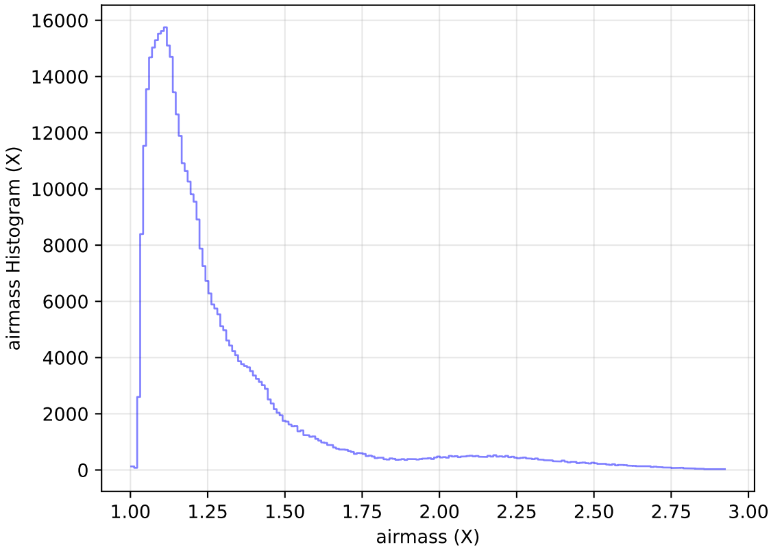
noroll_mjdp365_v3.4_10yrs WFD z band: airmass Histogram
