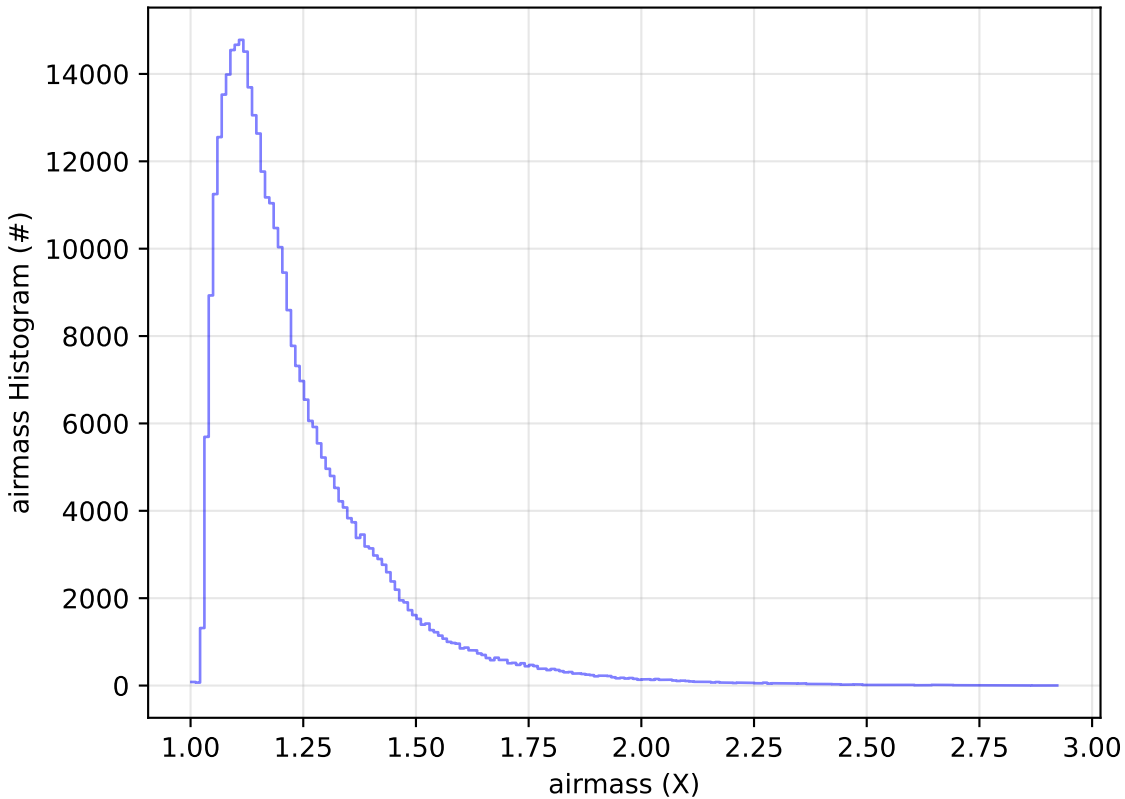
noroll_mjdp365_v3.4_10yrs WFD y band: airmass Histogram
