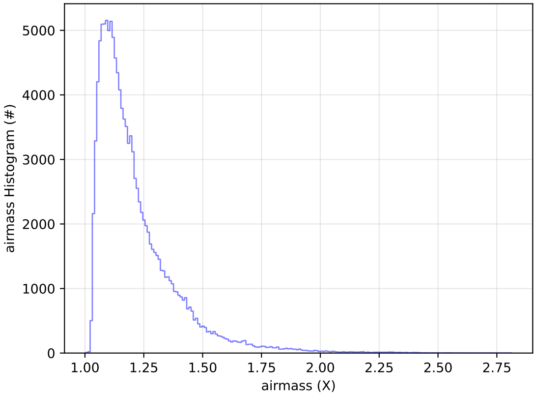
noroll_mjdp365_v3.4_10yrs WFD u band: airmass Histogram
