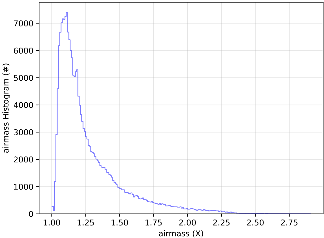
noroll_mjdp365_v3.4_10yrs WFD g band: airmass Histogram
