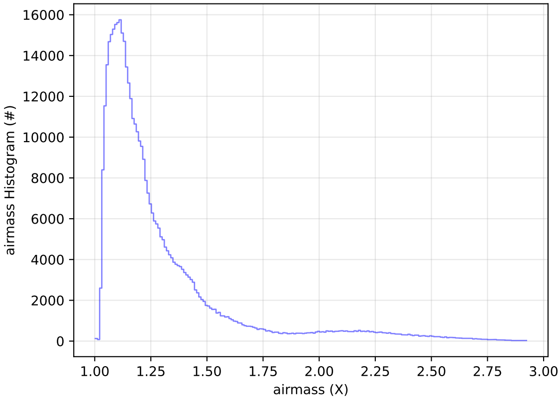
noroll_mjdp365_v3.4_10yrs All sky z band: airmass Histogram
