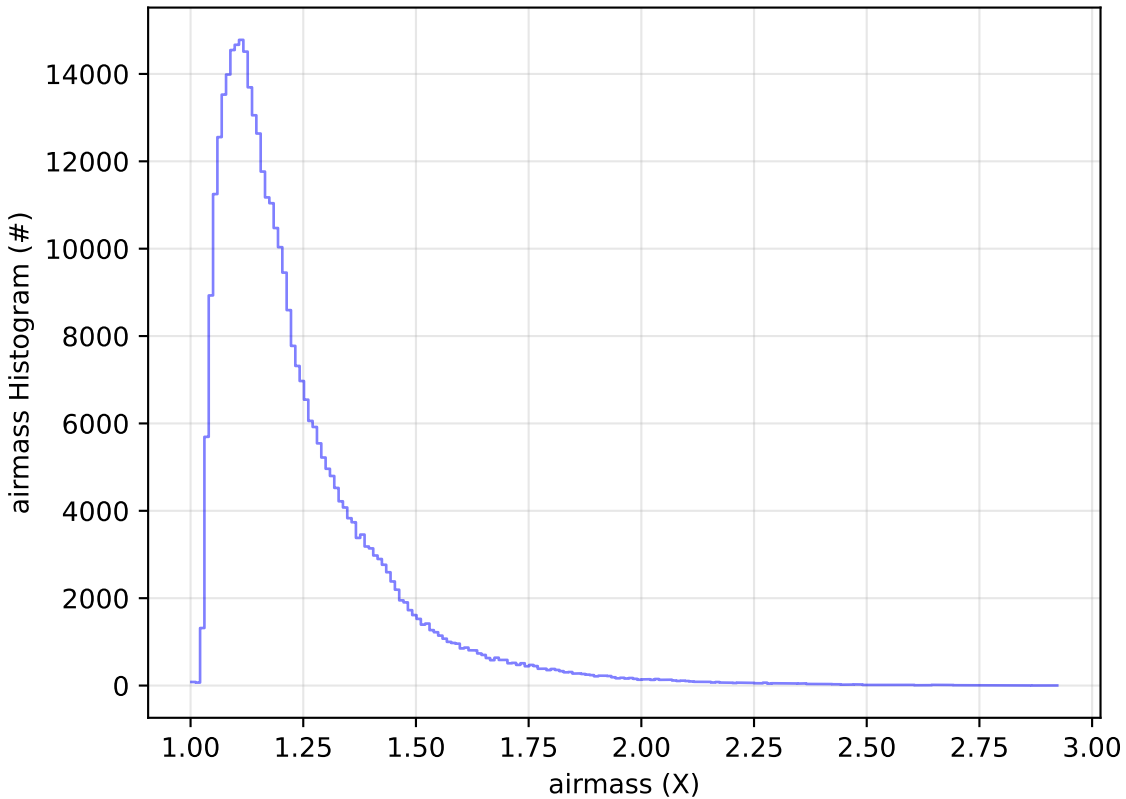
noroll_mjdp365_v3.4_10yrs All sky y band: airmass Histogram
