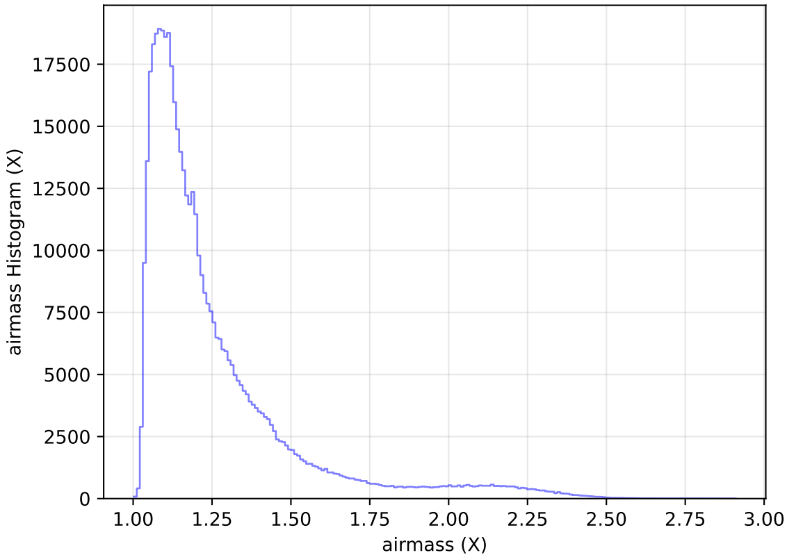
noroll_mjdp365_v3.4_10yrs All sky r band: airmass Histogram
