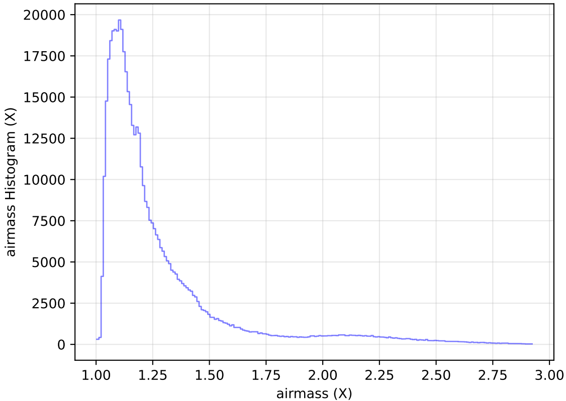
noroll_mjdp365_v3.4_10yrs All sky i band: airmass Histogram
