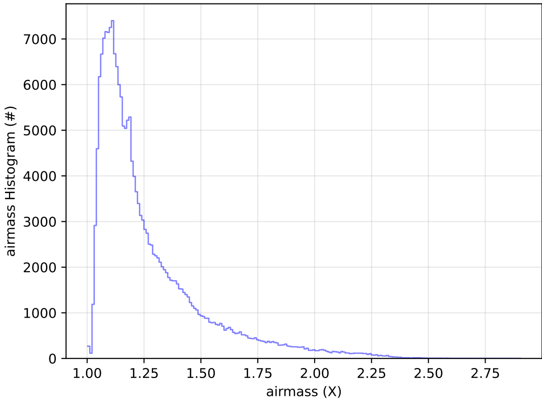
noroll_mjdp365_v3.4_10yrs All sky g band: airmass Histogram
