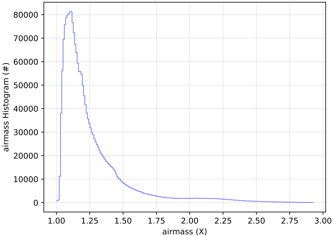
noroll_mjdp365_v3.4_10yrs All sky all bands: airmass Histogram
