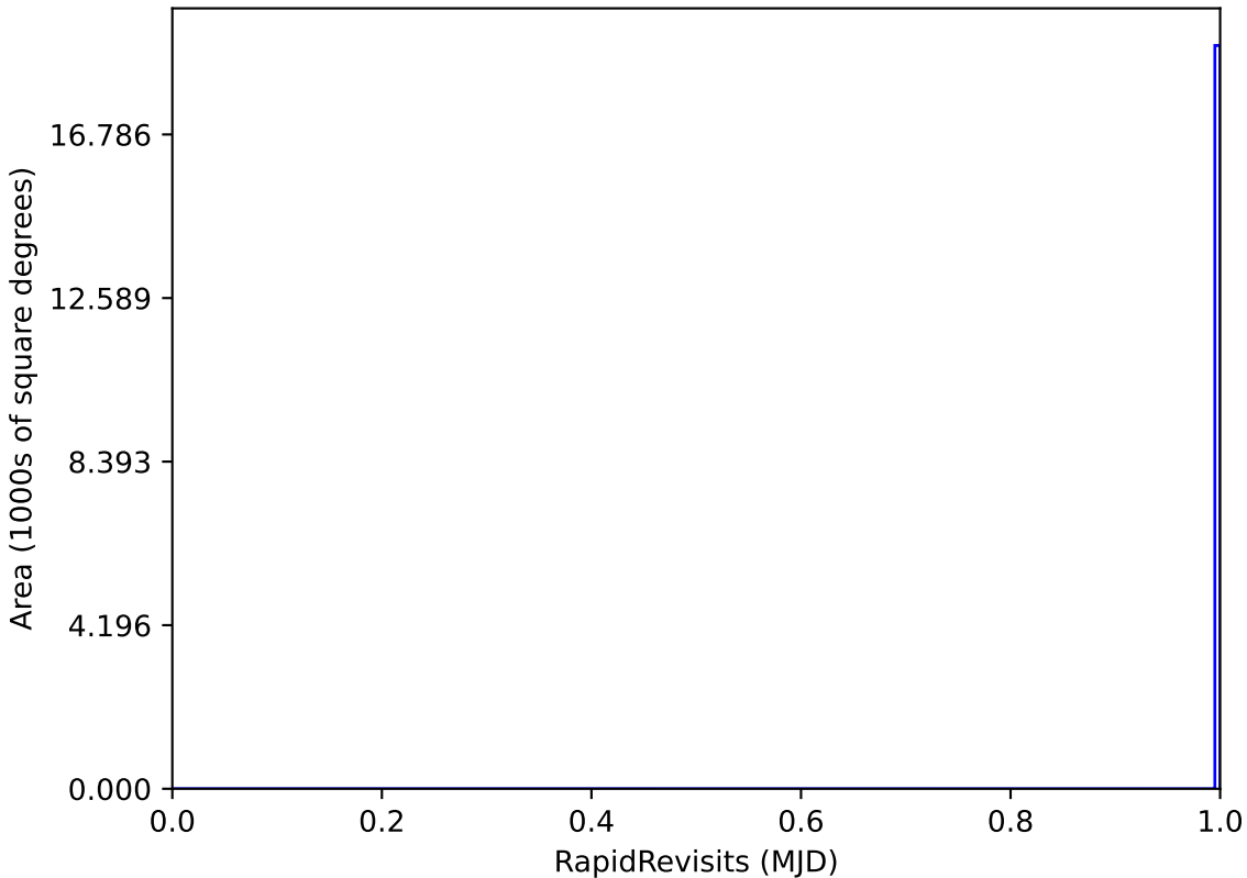
noroll_mjdp365_v3.4_10yrs WFD: RapidRevisits
