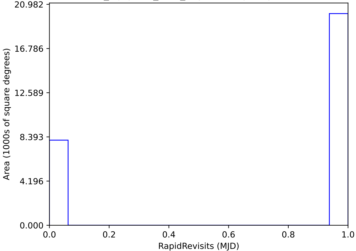
noroll_mjdp365_v3.4_10yrs All sky: RapidRevisits
