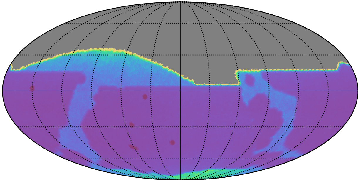
noroll_mjdp365_v3.4_10yrs All sky: Proper Motion Uncert @ 20.5
