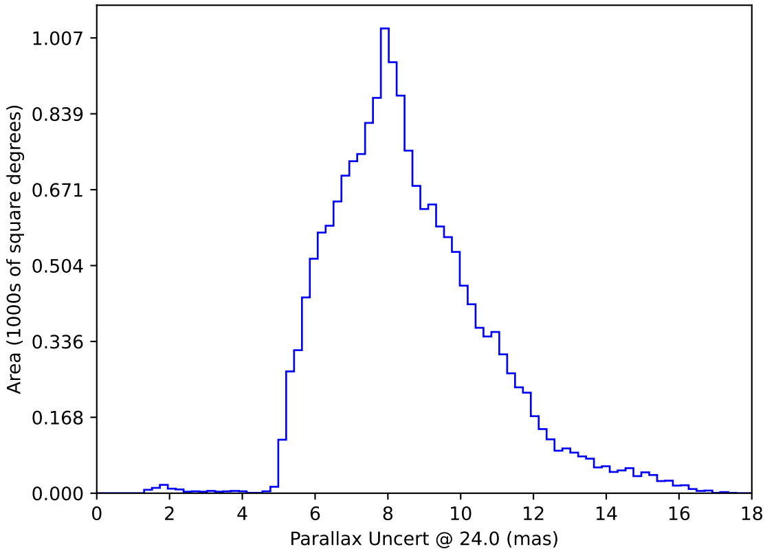
noroll_mjdp365_v3.4_10yrs WFD: Parallax Uncert @ 24.0
