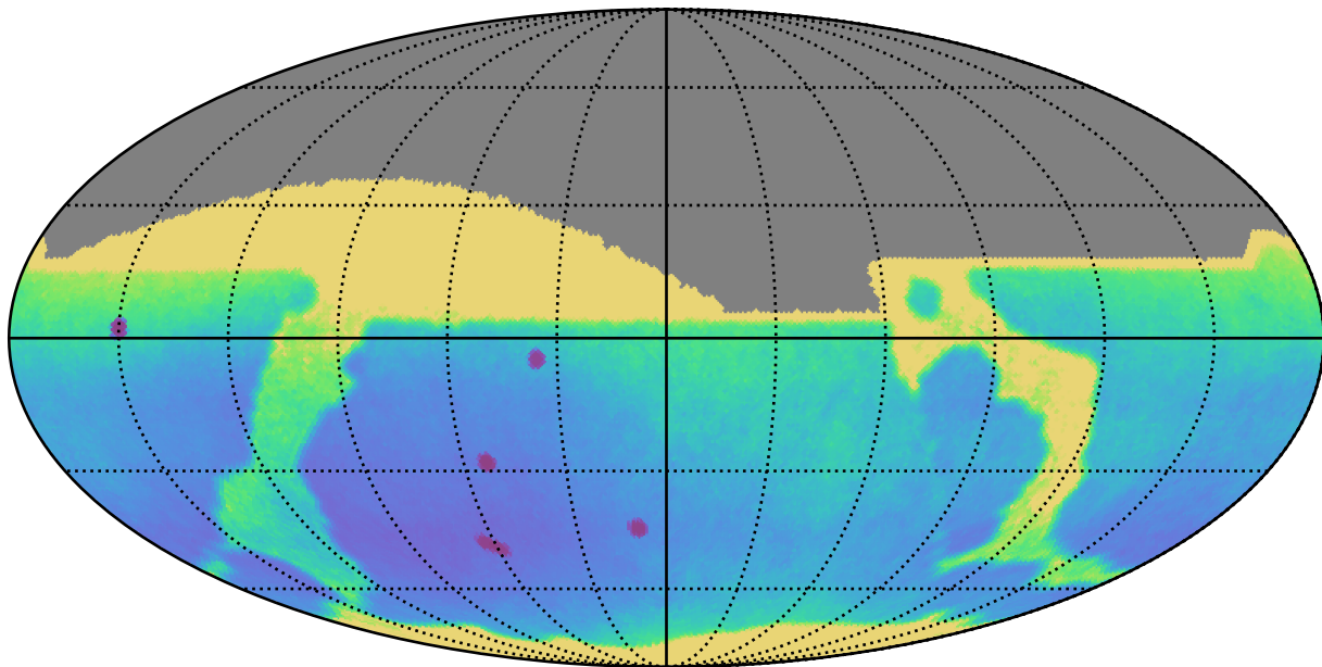
noroll_mjdp365_v3.4_10yrs All sky: Parallax Uncert @ 24.0
