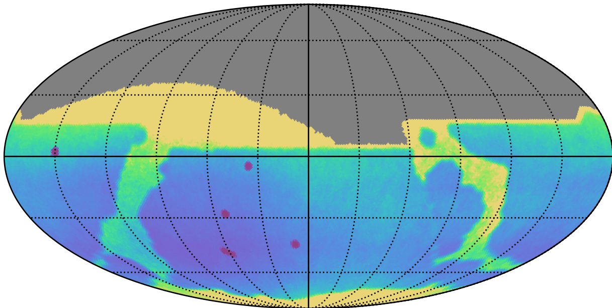
noroll_mjdp365_v3.4_10yrs All sky: Parallax Uncert @ 22.4
