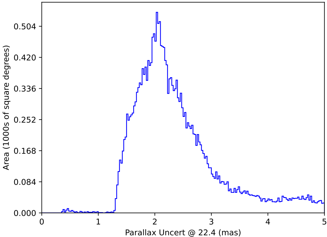
noroll_mjdp365_v3.4_10yrs All sky: Parallax Uncert @ 22.4
