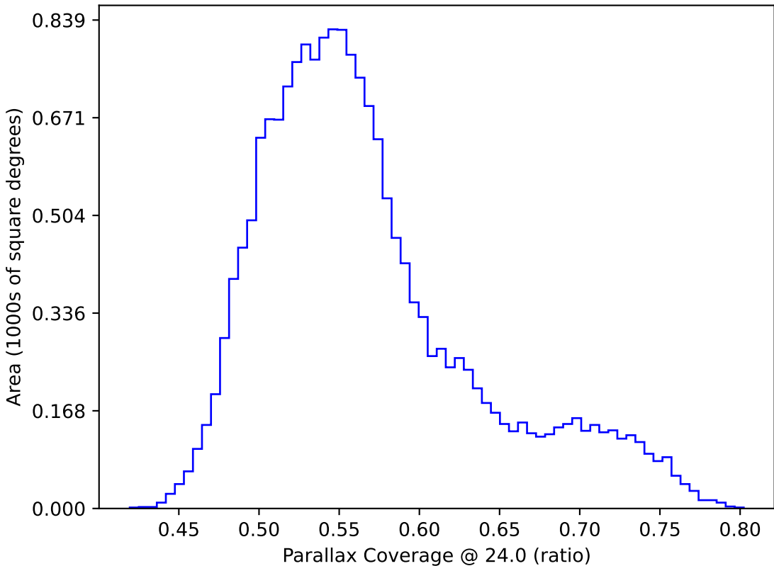
noroll_mjdp365_v3.4_10yrs WFD: Parallax Coverage @ 24.0
