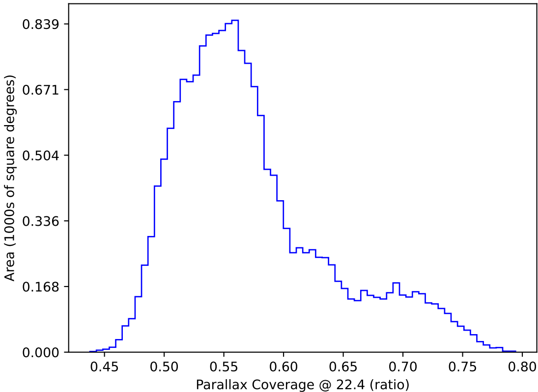
noroll_mjdp365_v3.4_10yrs WFD: Parallax Coverage @ 22.4
