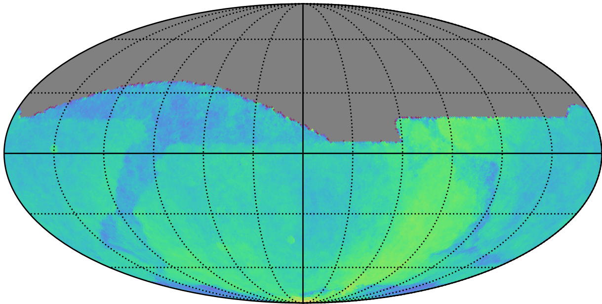
noroll_mjdp365_v3.4_10yrs All sky: Parallax Coverage @ 22.4
