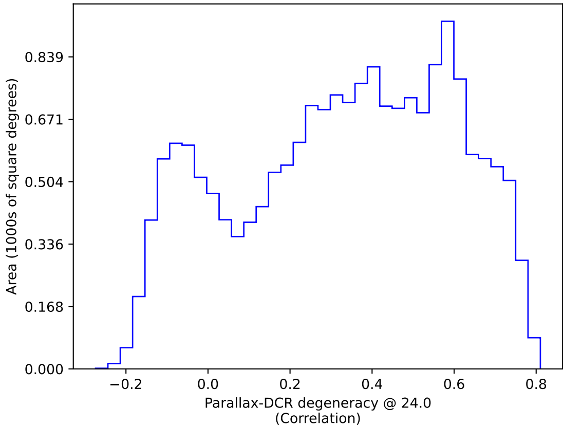
noroll_mjdp365_v3.4_10yrs WFD: Parallax-DCR degeneracy @ 24.0
