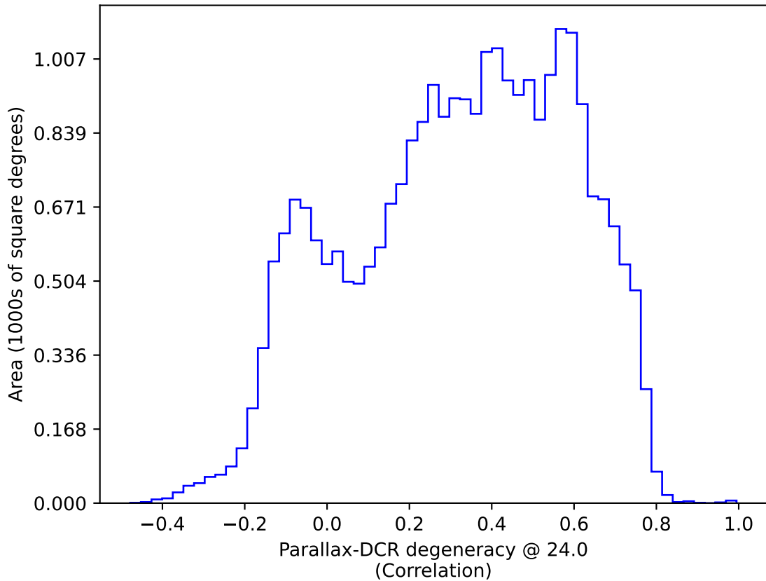
noroll_mjdp365_v3.4_10yrs All sky: Parallax-DCR degeneracy @ 24.0
